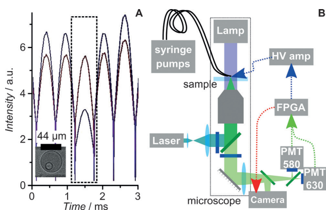
Figure 2. Detection of CTCs using a dual-emission SNARF 5F dye. A) Fragment of a raw data trace. The red/purple line shows fluorescence intensity monitoring at \lambda = 580 nm, the dark-blue line monitors at \lambda = 630 nm. Inset: micrograph of a detected CTC. B) Schematic of the experimental setup. PMT = photomultiplier; FPGA = field programmable gate array; HV amp = high-voltage amplifier.
