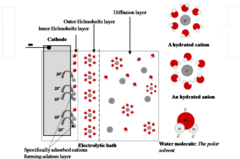
Figure 1. Illustration of a fundamental cathodic electrodeposition process at for a single constituent metal salt dissolved in an aqueous electrolyte
