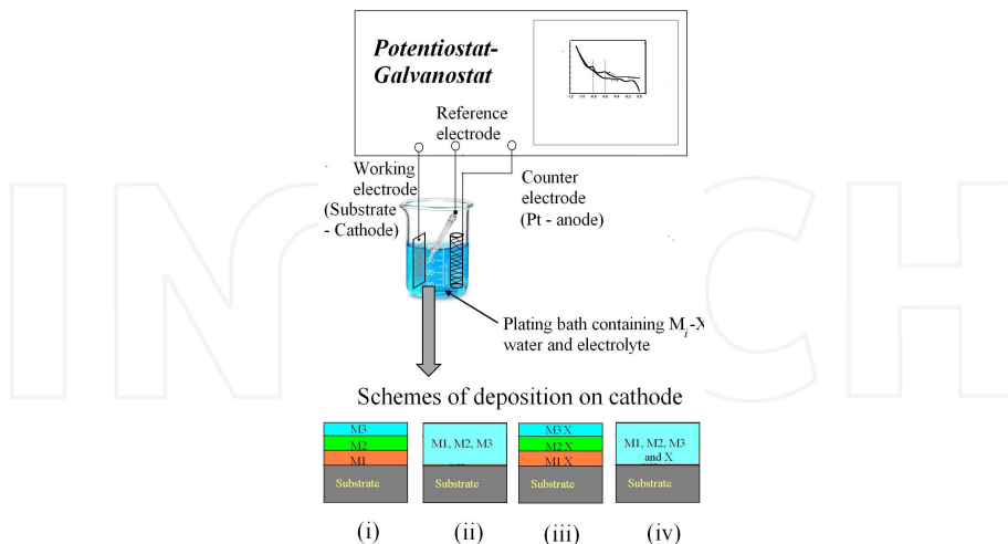
Figure 3. Schemes of cathodic electrodeposition of precursor film to be post annealed (EDA) for p-type photovoltaic absorber layers in literatures. Here, M_i represent constituent metal and X represents oxidized anion.
