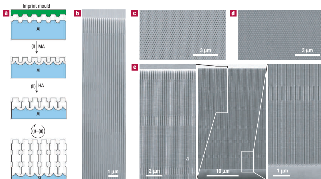
Figure 4 Long-range ordered alumina membranes with modulated pore diameters. a , Scheme for the fabrication of porous alumina with modulated pore diameters by a combination of MA and HA of a pre-patterned aluminium substrate. b , SEM micrograph showing a cross-section of anodic alumina ( D_{\text{int}} = 210 nm) with an ultra-high aspect ratio ( >1,000 ) of uniform nanopores; the HA on pre-patterned aluminium ( D_{\text{int}} = 210 nm) was conducted at 110 V. c,d , SEM micrographs showing the top and bottom surface view of the as-prepared anodic alumina ( D_{\text{int}} = 275 nm) with perfect hexagonal arrangement of the nanopores. e , SEM micrographs showing the cross-section view of the corresponding sample with modulated pore diameters. Magnified cross-section images of the top and bottom parts of the membrane are shown on the left and right, respectively.
