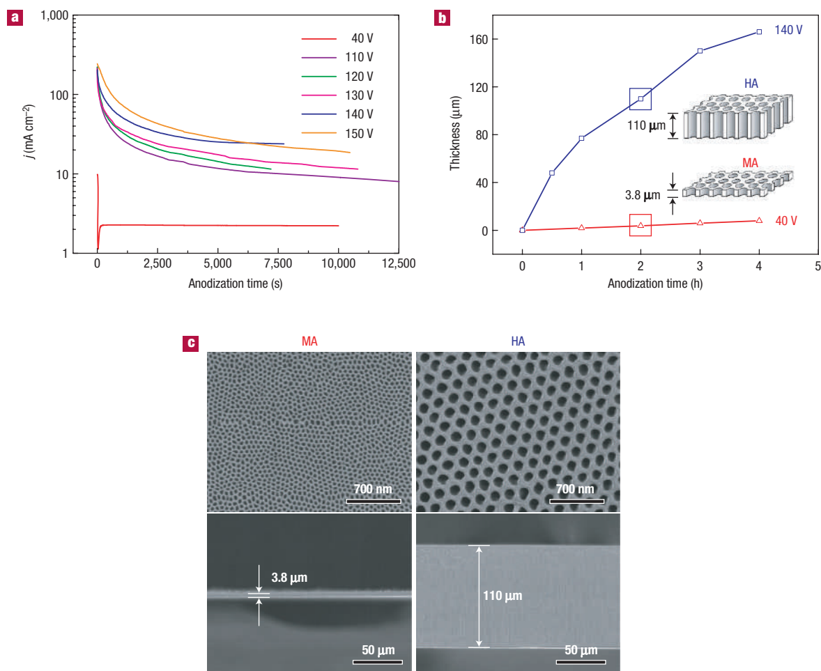
Figure 1 Hard anodization versus mild anodization. a , Current–time transients during HA of electropolished aluminium substrates in 0.3 M H 2 C 2 O 4 (1 °C). The current–time transient of a conventional MA (0.3 M H 2 C 2 O 4 , 1 °C, 40 V) is also plotted (red line) for comparison. b , Film thickness as a function of time during HA at 140 V (blue line) and an MA process at 40 V (red line). The different thicknesses of anodic oxides after 2 h of anodization are highlighted schematically in the insets. c , SEM micrographs of the corresponding AAO specimens formed by MA for 2 h (left column) and HA for 2 h (right column). The arrangements of pores for the respective samples are shown in the upper SEM micrographs. The thicknesses of the respective samples are indicated in the cross-sectional SEM micrographs.
