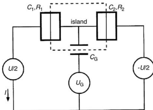
Figure 5.22 Circuit equivalent of a simple single-electron transistor, consisting of a two-junction arrangement and a gate electrode coupled capacitively to the central island. The
