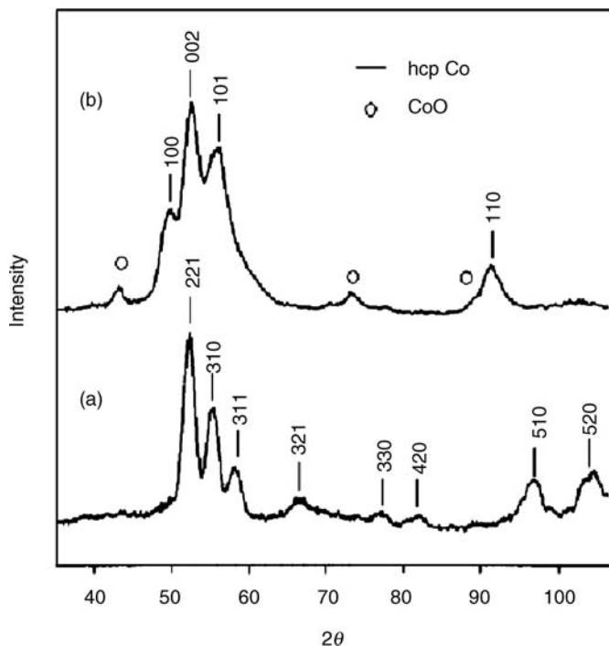
Figure 3.117 XRD patterns of the \epsilon -Co particles before and after annealing. (a) As-synthesized 9 nm particles; (b) After annealing at 300 °C under vacuum for 3 h. Reproduced with permission from Ref. [9]; © 1999, American Institute of Physics.
