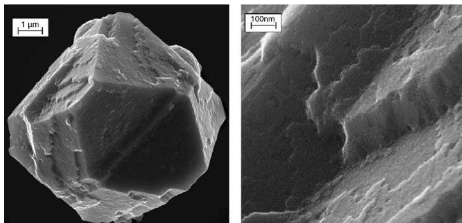
Figure 4.15 HR-SEM images of the surface of a CoPt 3 colloidal crystal.
