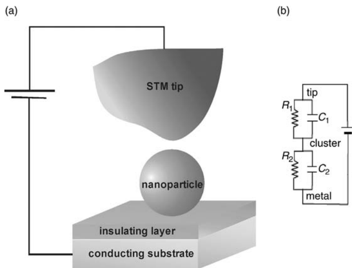
Figure 5.25 (a) General scheme of the STM configuration for the investigation of SET on individual metal nanoparticles; (b) Corresponding electronic circuit
