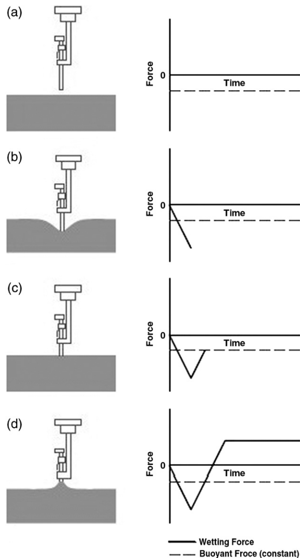
Fig. 12. Wetting balance technique of contact angle measurement [41].
