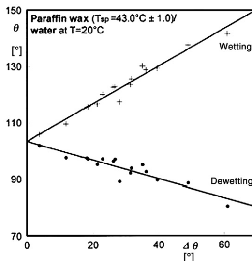
Fig. 9. Experiment of wetting/dewetting of water on paraffin wax surface [40].
