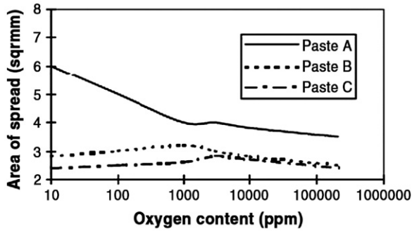
Fig. 26. Effect of atmosphere on area of spread of solder paste [66].
