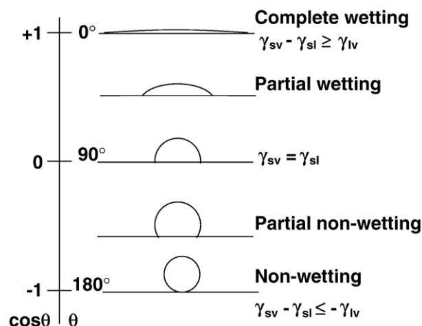
Fig. 4. Liquid drop on a solid substrate under various wetting conditions [23].
