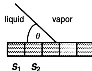
Fig. 17. Sessile drop placed on a composite surface [65].
