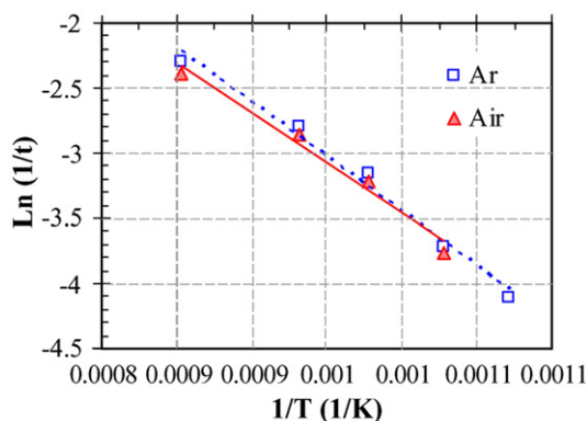
Fig. 23. Determination of activation energy for spreading [10].
