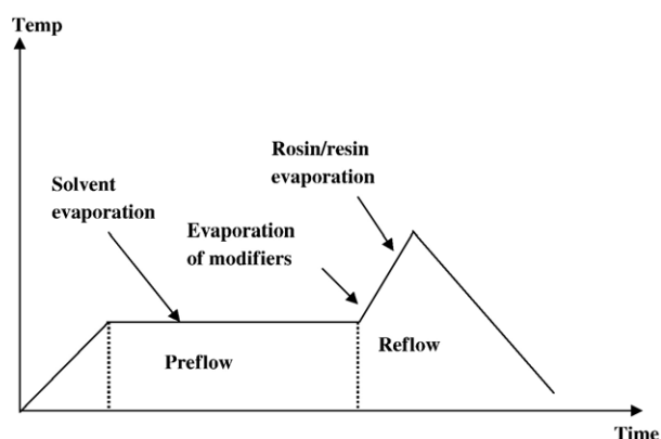
Fig. 20. Reflow soldering profile [66].
