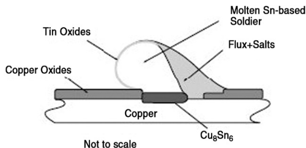
Fig. 19. Action of flux altering the wetting phenomenon [7].
