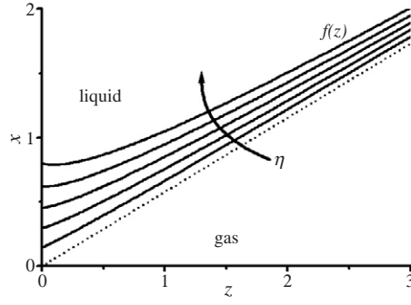
Figure 6. Equilibrium surface profiles ( \theta = 60^\circ ; \eta = 0.2, 0.4, \dots, 1.0 ; \varepsilon_d = 1 ). Reprinted with permission from Buehrle et al [43]. Copyright 2003 by the American Physical Society.
