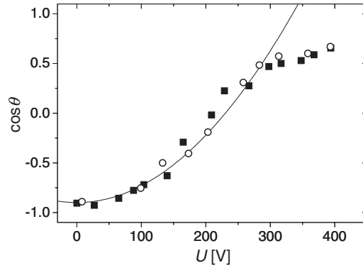
Figure 3. Contact angle versus applied (RMS) voltage for a glycerol–salt (NaCl) water droplet (conductivity: 3 \text{ mS cm}^{-1} ; AC frequency: 10 \text{ kHz} ) with silicone oil as the ambient medium. Insulator: Teflon AF 1601 ( d \approx 5 \text{ }\mu\text{m} ). Note that \theta_Y is almost 180^\circ for this system. Filled (open) symbols: increasing (decreasing) voltage. Solid line: parabolic fit according to equation (8) (reproduced from [52]).
