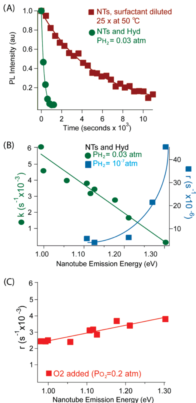
Figure 5. (A) PL emission intensity for the (7,6) nanotube as a function of time after CaHydI is added to the SWNT suspension (circles) and a pure SWNT suspension (no CaHydI) is diluted 25-fold and heated to 50 °C (squares). (B) Individual nanotubes' rate of PL bleaching upon CaHydI addition ( k , circles) and the rate of PL return when the H_2 partial pressure is reduced ( r , squares) versus nanotube emission energy. (C) Individual nanotubes' rate of PL recovery ( r ) upon exposure to atmospheric O_2 versus nanotube emission energy. The rates are obtained by fitting the progress curve data for each nanotube to first-order exponential functions. The lines in (A) are fit exponential functions and the lines in (B) and (C) are guides to the eye. (For more detailed explanation see "kinetic model" in Supporting Information).
