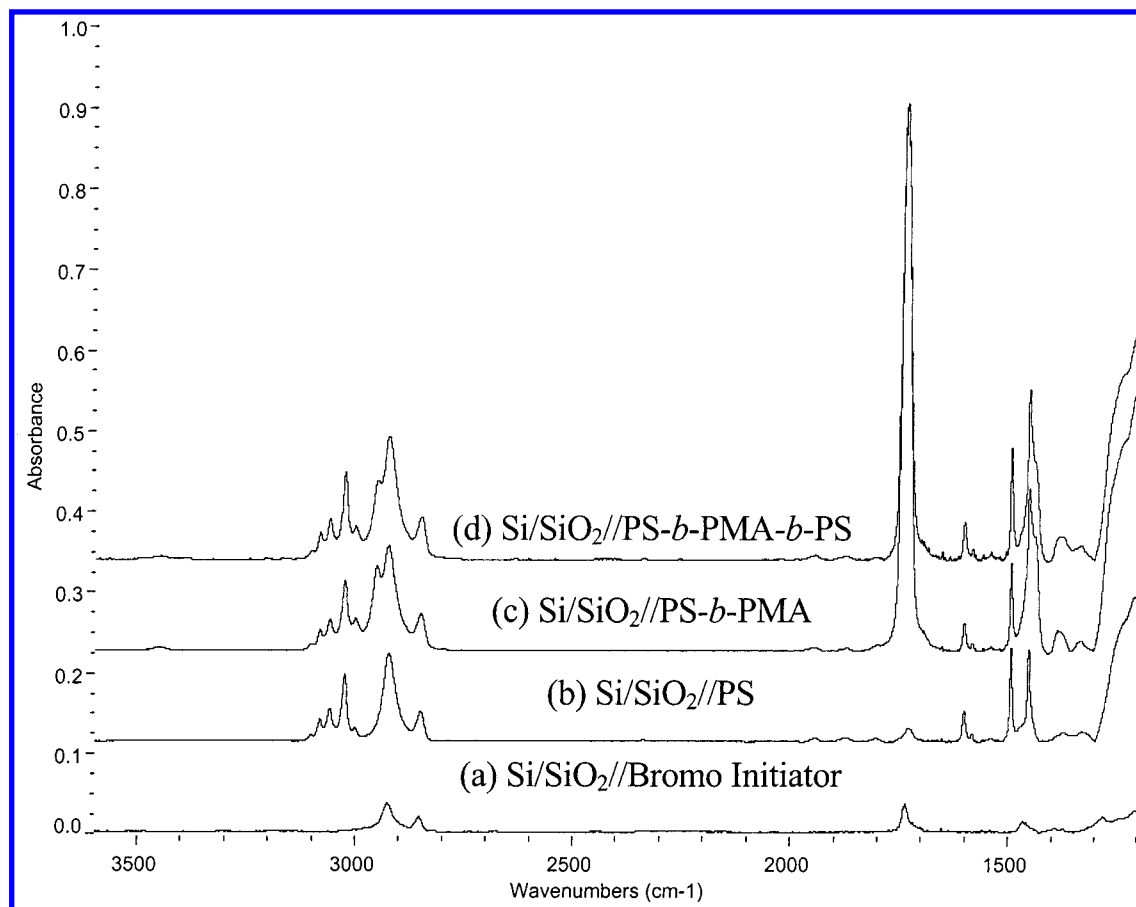
Figure 2. ATR-FTIR spectra of (a) Si/SiO 2 /bromo-isobutyrate initiator, (b) Si/SiO 2 /PS (tethered PS brush), (c) Si/SiO 2 /PS- b -PMA, and (d) Si/SiO 2 /PS- b -PMA- b -PS.
