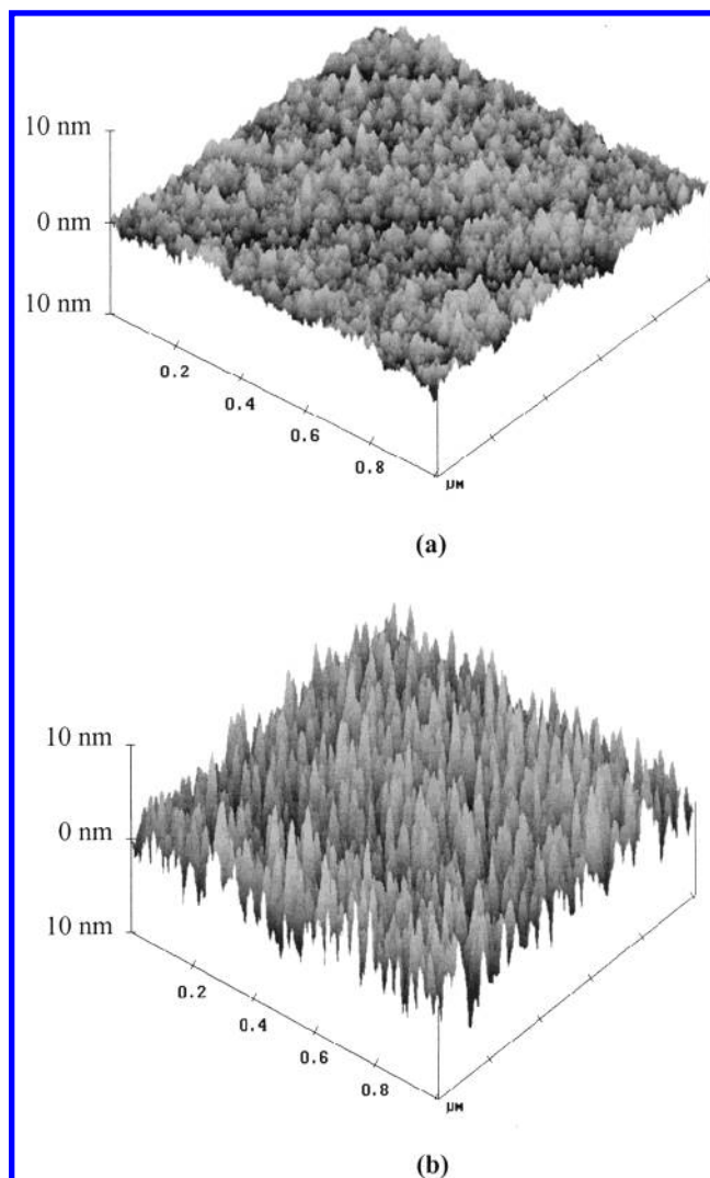
Figure 5. AFM images of Si/SiO 2 //PS- b -PMA- b -PS brush (a) after treatment with CH 2 Cl 2 and (b) after treatment with acetone.
