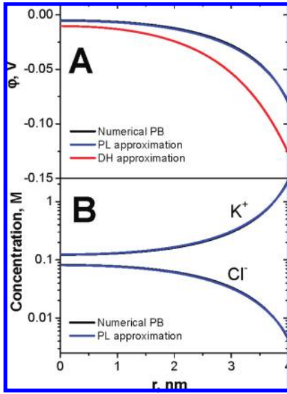
Figure 2. Radial distributions inside a long cylindrical nanochannel of radius a = 4 nm and surface charge density \sigma = -0.5\text{e/nm}^2 with bulk concentration C_{\text{bulk}} = 0.1 M for (A) the electric potential, \phi , calculated using DH approximation (red line), analytical PL approximation for PB (blue line), and direct numerical calculations using PB (black line), which practically coincide. (B) Profiles of \text{K}^+ and \text{Cl}^- concentrations.
