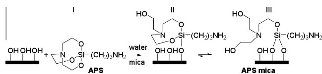
Fig. 3. Scheme of mica modification by 1-(3-aminopropyl)silatrane. APS (I) reacting with the hydroxyl groups of mica, forming a transient molecule (II), and yielding a product (III).
