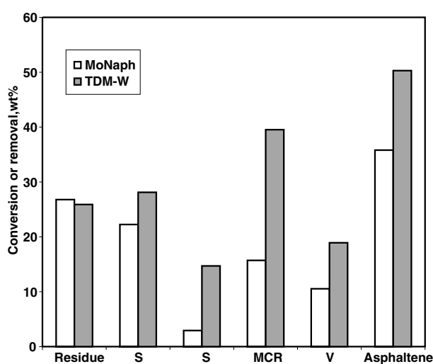
Figure 2. Cold Lake bitumen upgrading using MoS 2 derived from molybdenum naphthenate (MoNaph) and exfoliated MoS 2 dispersed in water (TDM-W) (Reaction conditions: 415 °C at an initial H 2 pressure of 3.5 MPa and a reaction time of 1 h with 600 ppm Mo.)
