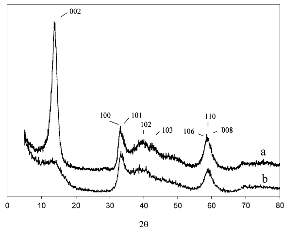
FIG. 3. X-ray diffraction diagrams of unsupported molybdenum sulfides; (a) aqueous \text{MoS}_2 ; (b) MD \text{MoS}_2 .
