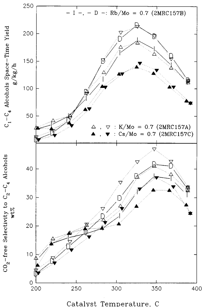
Figure 7. Catalytic performances of the molybdenum sulfide catalyst of Figure 4, part a, when doped with various alkali metals. (Alkali:Mo = 0.7:1). Symbols used for increasing-temperature and decreasing-temperature legs, respectively: K-doped, open upward triangle and open downward triangle; Rb-doped, I and D; Cs-doped, filled upward triangle and filled downward triangle. Amounts of catalysts used: K-doped, 0.53 g; Rb-doped, 0.51 g; Cs-doped, 0.51 g. Other reaction conditions are as those in Figure 4, part a.
