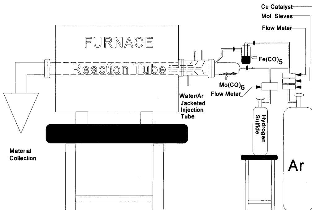
Figure 1. Schematic of apparatus used for synthesis of molybdenum sulfide by vapor-phase reduction of molybdenum carbonyl.
