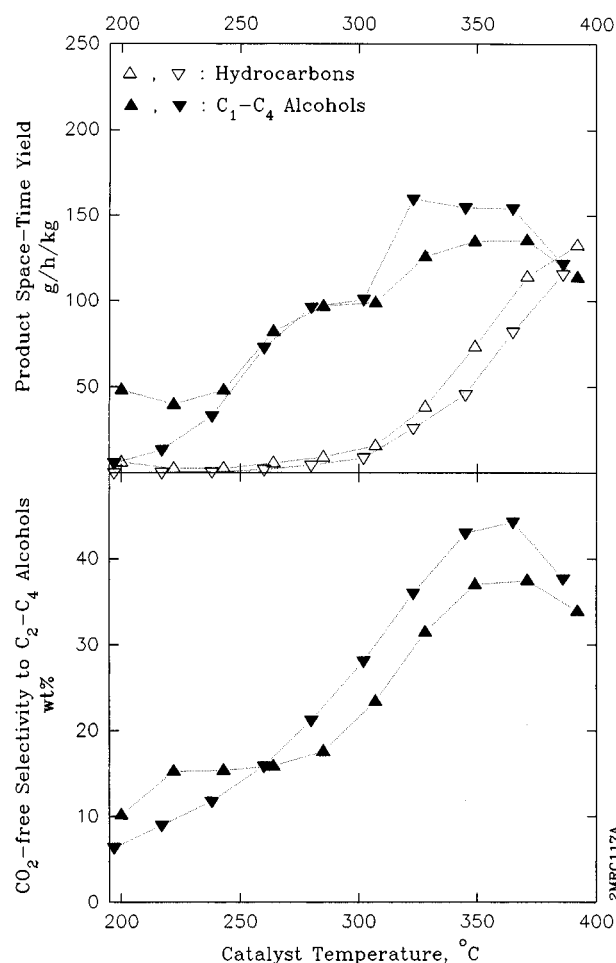
Figure 10. Performance of K-doped catalyst similar to that in Figure 5, except that the molybdenum sulfide was synthesized at a furnace temperature, T_h , of 600 °C.
