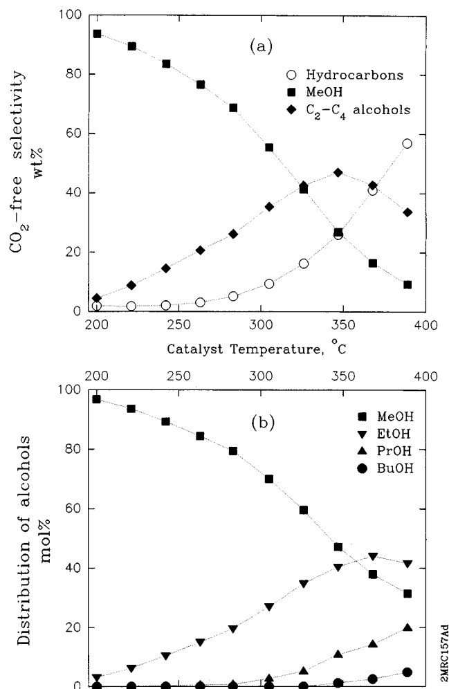
Figure 6. Selectivities of the K-doped molybdenum sulfide catalyst of Figure 5.
