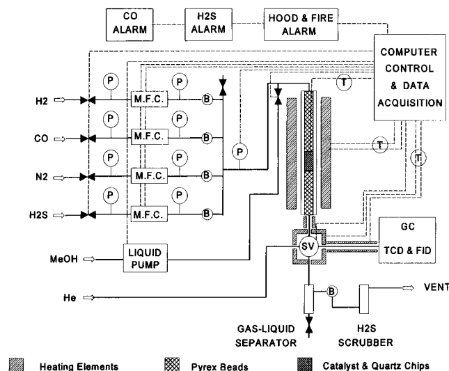
Figure 3. Schematic of apparatus for catalytic reactions: SV, sample valve; MFC, mass flow controller; P, pressure gauge; T, thermocouple; B, back-pressure regulator.
