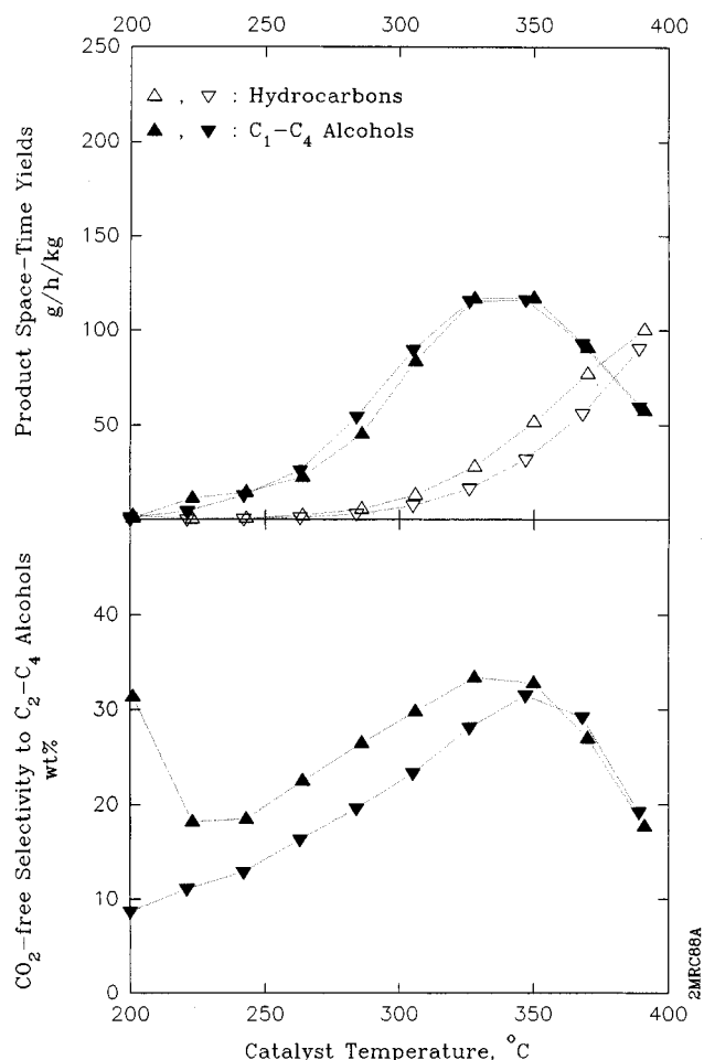
Figure 11. Performance of K-doped catalyst essentially similar to that in Figure 5 after dilution with silica. Symbols are the same as those in Figure 4, part a.
