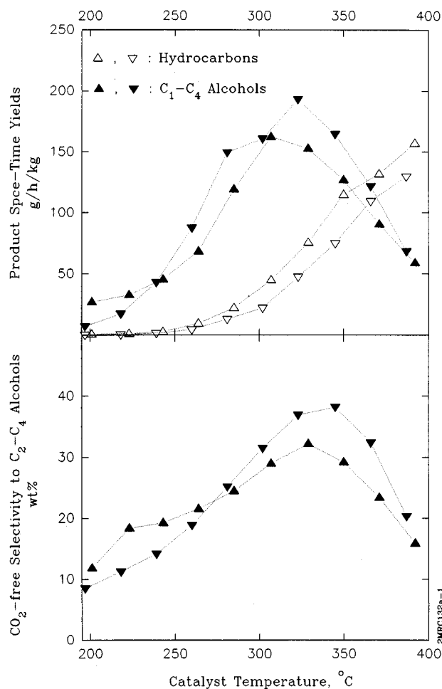
Figure 9. Performance of Cs-doped catalyst similar to that in Figure 8, except that the molybdenum sulfide was synthesized at a furnace temperature, T_h , of 400 °C (sample 2MRC129A in Table 1).
