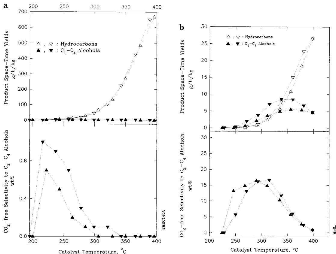
Figure 4. (a) Results of base line screening run on undoped molybdenum sulfide synthesized by VPR at the "standard" conditions ( T_f = 500 °C and other conditions of Table 1). Reaction conditions: 0.48 g of catalyst, P = 750 psig, GHSV = 6000 L/kg/h, H_2/CO = 1:1 . Upward-pointing and downward-pointing triangles are the data for the temperature-increasing and temperature-decreasing legs, respectively. Filled and open symbols refer to alcohols and hydrocarbons, respectively. (b) Results of base line screening run on commercially available molybdenum sulfide. Symbols and reaction conditions are as those in (a), except that 0.50 g of catalyst was used.
