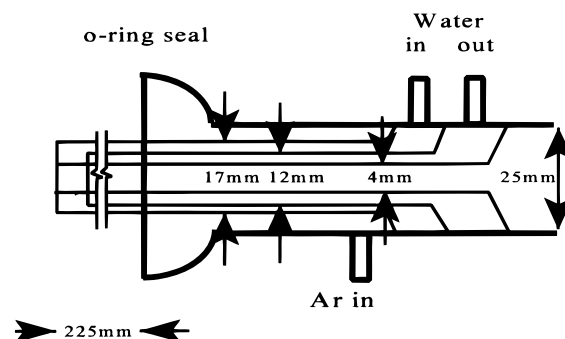
Figure 2. Detail of injector tube cooled by water and argon as used in the apparatus of Figure 1.
