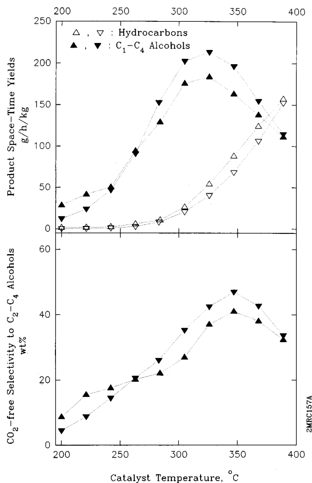
Figure 5. Results when the molybdenum sulfide of Figure 4, part a, is doped with potassium (K:Mo = 0.7:1). Reaction conditions are as those in Figure 4, part a, except that the weight of catalyst used is 0.53 g. Symbols are as those in Figure 4, part a.
