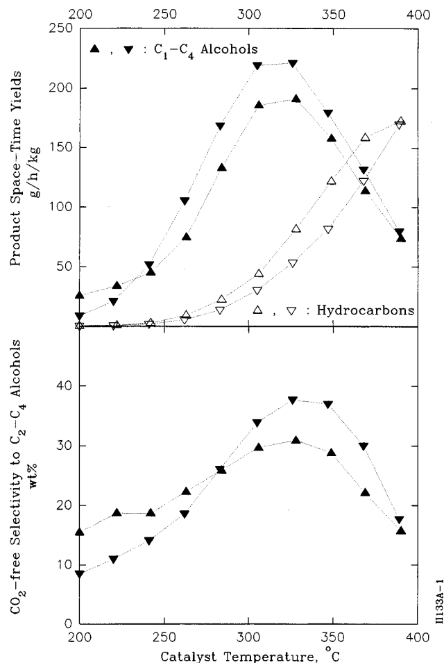
Figure 8. Catalytic performance of the alkali-doped molybdenum sulfide when Cs:Mo = 0.22:1. Symbols and reaction conditions are as in Figure 4, part a. Amount of catalyst used is 0.4 g.
