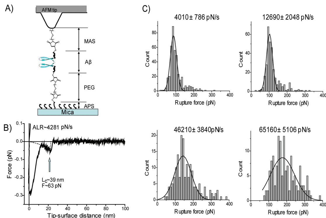
Figure 1. (A) Schematic experimental system of SMFS. The AFM tip and mica surface were functionalized with MAS and A \beta -40 and with APS, PEG, and A \beta -40, respectively. In the schematic, A \beta s are shown as \beta -hairpin structures in dimeric form. (B) Representative force–distance curve measured at pH 5 with an apparent loading rate (ALR) of 4280 pN/s. (C) Histograms of the rupture force distribution measured at pH 5 at ALRs of 4000, 12690, 46210, and 65160 pN/s. The most probable rupture forces ( F_r ) for each loading rate were \sim 88 , \sim 102 , \sim 143 , and \sim 177 pN, respectively, which were calculated by Gaussian fitting.
