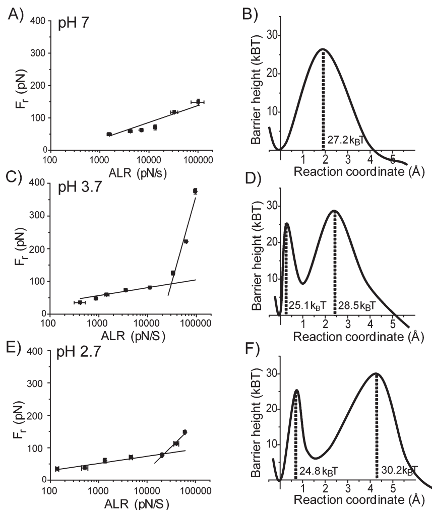
Figure 3. Results of the dynamic force spectroscopy analysis for different pH values. Each pair consists of the DFS plot and the corresponding profile of the energy landscape at pH 7 (A and B), pH 3.7 (C and D), and pH 2.7 (E and F). In the energy landscapes, the first valley is for the bound state, the second is for the intermediate, and the last is for the dissociation state of A \beta -40 dimers. The potential barrier heights were calculated using K_{\text{off}} (see the text) extracted from the linear fitting of Bell's model in the plot of F_r vs \ln(\text{ALR}) . All parameters used for energy landscapes are listed in Table 1.
