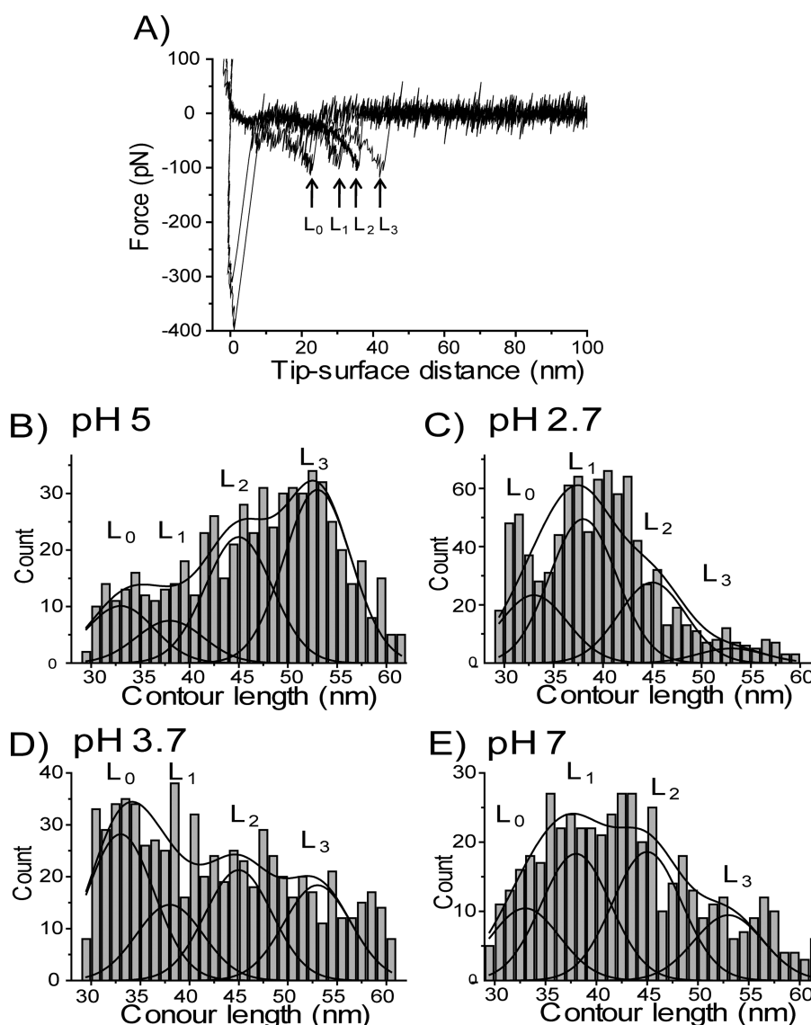
Figure 4. (A) Representative force curves for rupture events with different rupture lengths obtained at pH 5. All force curves were obtained at the same ALR regime ( \sim 34 nN/s) and correspond to rupture forces of \sim 120 pN. (B–E) Histograms of the contour length distributions measured at pH 5 (B), 2.7 (C), 3.7 (D), and 7 (E). Each histogram is approximated with four Gaussian curves with centers located around 33 ( L_0 ), 38 ( L_1 ), 45 ( L_2 ), and 53 nm ( L_3 ). The data were collected over the pulling rate range from 0.1 to 10 nN/s.
