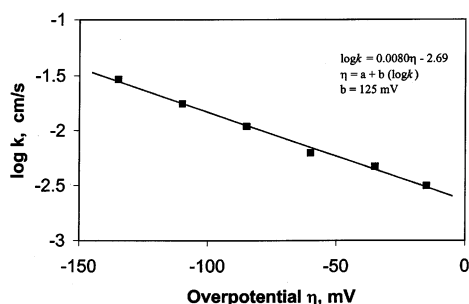
Figure 11. Tafel plot of O_2 reduction on platinum.
