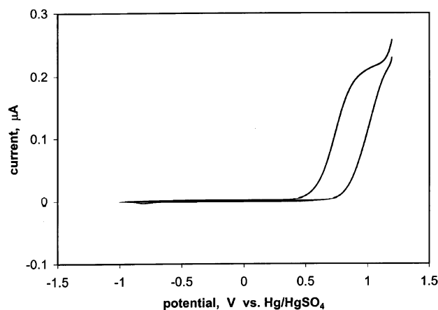
Figure 5. CV recorded with a platinum microelectrode of 25 \mu\text{m} diameter in a solution of 10 mM sodium hydroxide and 0.1 M \text{Na}_2\text{SO}_4 at 100 mV/s.
