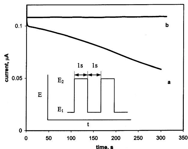
Figure 6. Plot of limiting current against time for a 12.5 \mu\text{m} radius Au microelectrode held at a constant potential (1.2 V) (a) and with a programmed potential (b). The solution was 5 mM in sodium hydroxide and 0.1 M in \text{Na}_2\text{SO}_4 . The inset shows the potential profiles for (b). E_1 was -0.9 V, and E_2 was 1.2 V.
