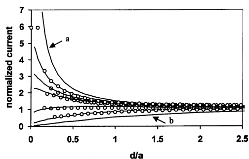
Figure 8. SECM approach curves. The solid lines a and b are theoretical approach curves at conducting and insulating substrates, respectively. Circle symbols are experimental approach curves, and solid lines are theoretical curves at a Pt substrate with its potential held at, from top to bottom, -0.9 , -0.8 , -0.7 , -0.6 , and -0.5\ \text{V} . Approach speed was 0.45\ \mu\text{m/s} . The tip was a 12.5\ \mu\text{m} radius Au microdisk. The solution contained 10\ \text{mM} sodium hydroxide and 0.1\ \text{M} in \text{Na}_2\text{SO}_4 . The two highest experimental points occurred with the -0.9\ \text{V} scan when the tip touched the substrate and were not used in the curve fitting.
