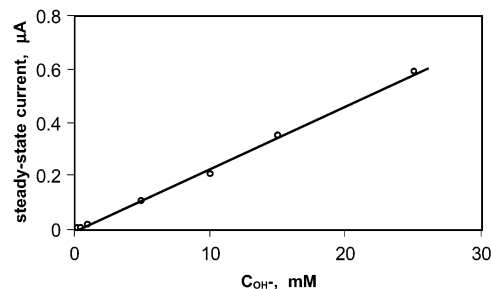
Figure 3. Steady state limiting current vs concentration of sodium hydroxide in aqueous solution containing 0.1 M \text{Na}_2\text{SO}_4 .
