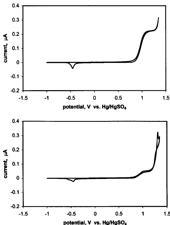
Figure 2. CVs for a 10 mM deaerated solution of sodium hydroxide, recorded with a freshly polished gold disk electrode of 25 \mu\text{m} diameter (a) or with the same electrode that was polarized at 1.2 V for 5 min (b). The solution contained 0.1 M \text{Na}_2\text{SO}_4 . The scan rate was 100 mV/s.
