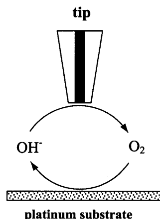
Figure 1. Feedback mode of SECM used in the study of \text{O}_2 reduction in alkaline solution.
