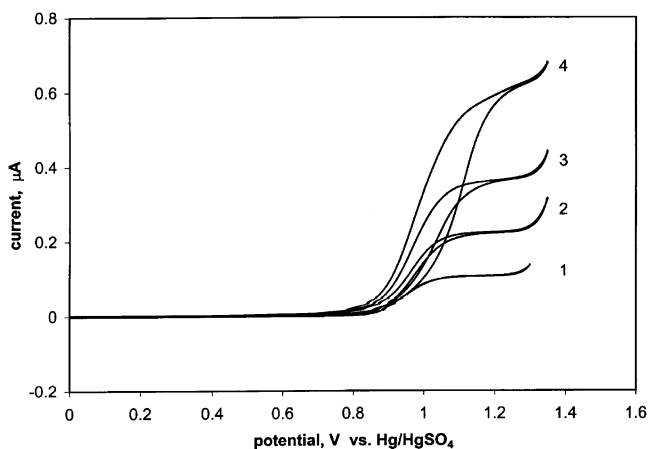
Figure 4. Voltammograms for hydroxide ion oxidation on a 25 \mu\text{m} diameter Au microelectrode in 0.1 M \text{Na}_2\text{SO}_4 solution. The scan rate was 100 mV/s. The concentration of hydroxide ion: (1) 5, (2) 10, (3) 15, and (4) 25 mM.
