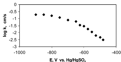
Figure 10. Heterogeneous reaction rate constant k of O_2 reduction at a Pt substrate with different potentials. k was obtained by fitting the experimental approach curves with the theoretical ones as shown in Figure 8.
