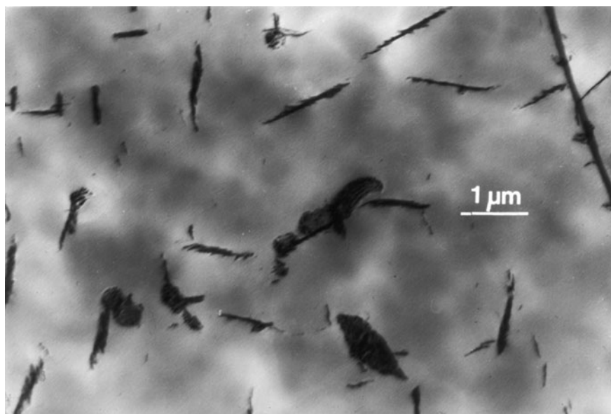
Fig. 11.23 Precipitation of \alpha'' -Fe 16 N 2 iron-nitride platelets along dislocation lines in an Fe–N solid solution (taken from Straver WTM, Rozendaal HCF, Mittemeijer EJ (1984) Metallurgical Trans A 15A:627–637)
