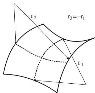
Fig. 10.17 A curved grain-boundary segment with its two principal radii of curvature r_1 and r_2 . At the position shown r_1 = -r_2 and, consequently, the corresponding, local pressure on the grain interior is nil, a situation which always occurs in the case of flat grain boundaries
