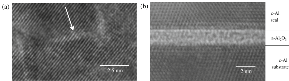
Fig. 6.19 (a) VN precipitate in an \alpha -Fe (b.c.c., ferrite) matrix. The 110 lattice fringes become curved due to lattice distortion caused by coherency stresses (taken from Vives Díaz NE, Hosmani SS, Schacherl RE, Mittemeijer EJ (2008) Acta Materialia 56:4137–4149). (b) Amorphous \text{Al}_2\text{O}_3 layer grown onto Al substrate with a {111} surface, formed during initial stage of oxidation in oxygen. The sample was afterwards sealed by an Al layer on top for protection of the oxide layer (taken from Reichel F, Jeurgens LPH, Richter G, Mittemeijer EJ (2008) J Appl Phys 103:093515)
