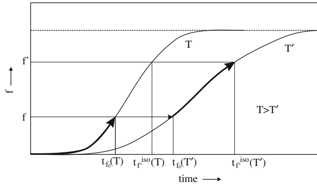
Fig. 9.40 Illustration of the “additivity” rule: Annealing for the time t_{f_0}(T) at temperature T and subsequent annealing for the time t_{f'}^{iso}(T') - t_{f_0}(T') at T' leads to the same degree of transformation f' as annealing for t_{f'}^{iso}(T') at T'
