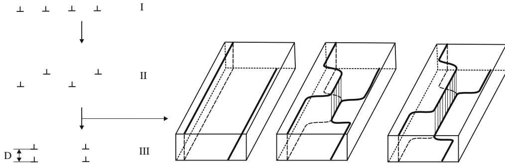
Fig. 10.5 (Edge) Misfit dislocations originally located in the interface of an A/B bicrystal ( top part of left part of the figure; see “I”) upon annealing can move away from the interface by climb (see “II”) and, subsequently, by glide can become aligned on top of each other (see “III”). A schematic depiction of this alignment process is shown in the right part of the figure: the dislocations align part by part. Thus dislocation walls can be formed initially comprising only two dislocations. Such observations have been made for Cu/Ni bicrystals (Beers and Mittemeijer, 1978)
