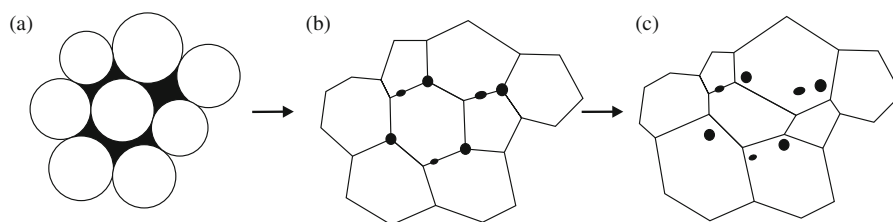
Fig. 5.28 Pores during the sintering process of powders. (a) and (b) Pores (black) are the relicts of the spaces between the original powder particles (white) and thus normally located at grain boundaries. (c) In late stages of sintering, grain growth may occur, during which the grain boundaries move away from the pores, leaving them in the interior of the grain
