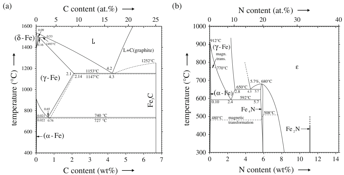
Fig. 9.22 Phase diagrams of (a) Fe-C and (b) Fe-N (redrawn from Massalski TB (Editor in Chief) (1996) Binary alloy phase diagrams, 2nd edn. ASM, Metals Park, OH)
