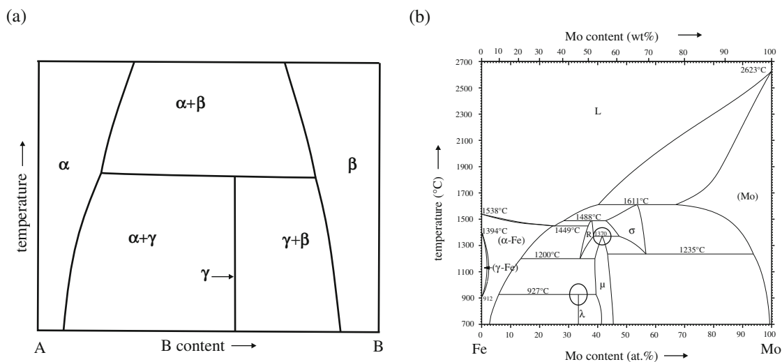
Fig. 7.24 (a) Schematic phase diagram of a binary system with a peritectoid reaction. (b) The Fe–Mo phase diagram (redrawn from Massalski, 1996); two peritectoid reactions, R + \sigma \leftrightarrow \mu and (\alpha\text{-Fe}) + \mu \leftrightarrow \lambda , have been marked by circles
