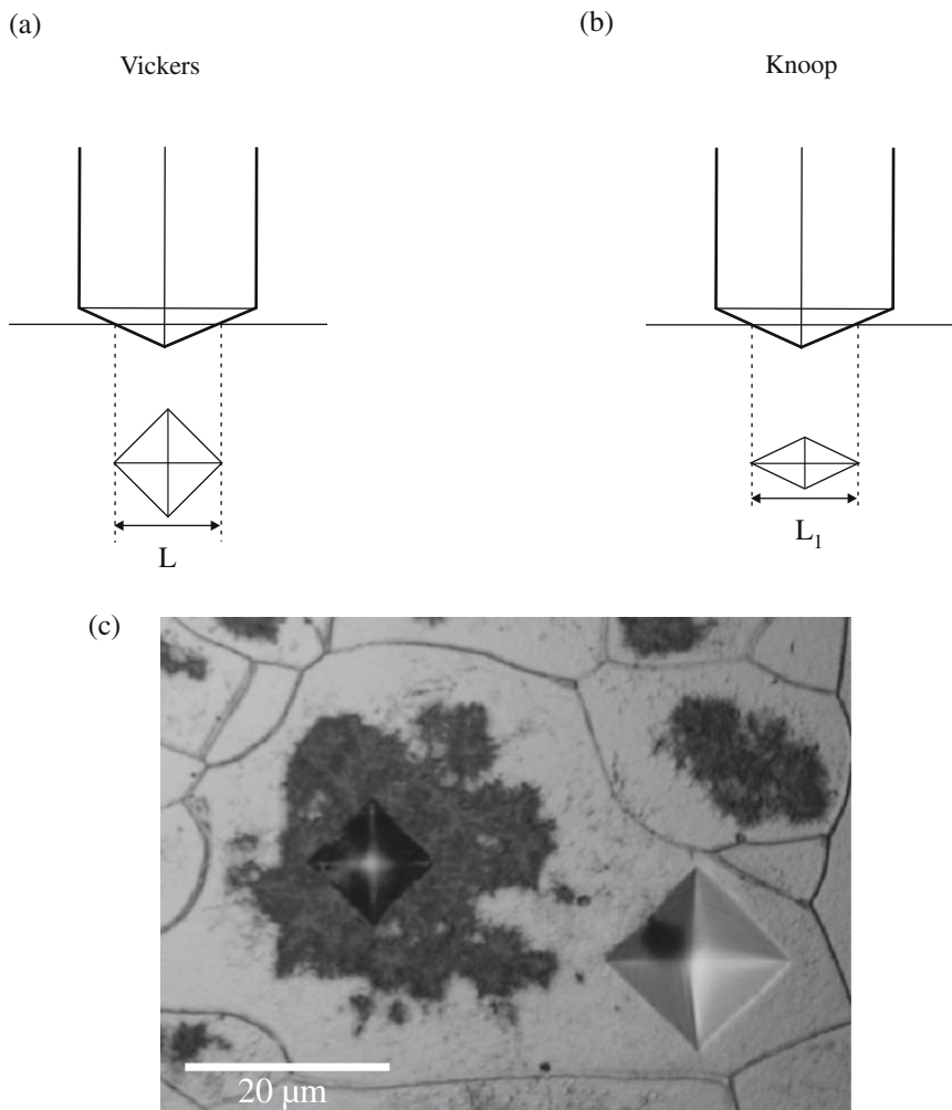
Fig. 11.34 Schematic illustration of (a) a Vickers and (b) a Knoop hardness indent. (c) Two (Micro)Vickers hardness indents in a grain of nitrided Fe-4.65 at.%Al alloy are shown (SEM image). In the grain interior a higher hardness than near the grain boundaries prevails (cf. the differently sized indents in the micrograph), because AlN precipitates have (already) developed in the grain interior (dark etching region; taken from and for more details see Meka S, Hosmani SS, Clauss AR, Mittemeijer EJ (2008) Int J Mater Res 99:808–814)
