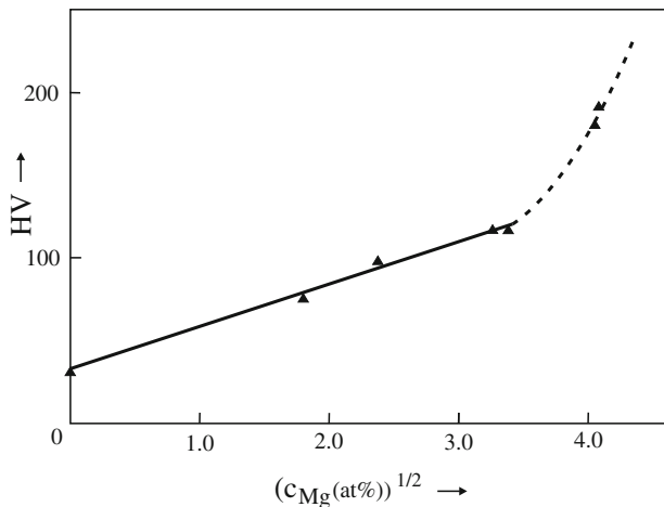
Fig. 11.46 Hardness (Vickers; cf. Sect. 11.13) as a function of Mg content for AlMg alloy specimens prepared by melt-spinning. A linear dependence of the hardness on (c_{\text{Mg}})^{1/2} is observed (solid solution hardening; full line ). The extraordinary increase in hardness for high Mg content ( >12 at.% Mg; dashed line ) is not due to solid solution hardening, but is attributed to the formation of Guinier–Preston zones (cf. Sects. 9.4.1 and 11.14.4) (redrawn from van Rooyen M, Colijn PF, de Keijser Th, Mittemeijer EJ (1986) J Mater Sci 21:2373–2384)
