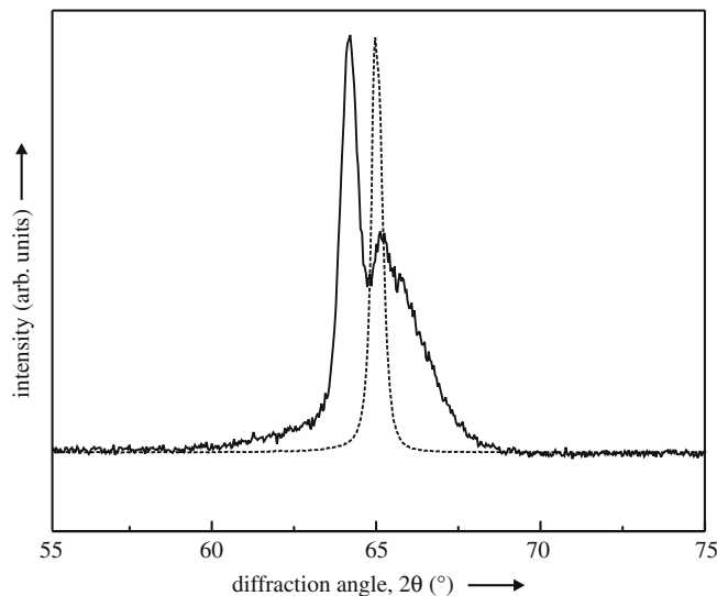
Fig. 5.26 Dashed line: \alpha -Fe-200 X-ray diffraction line profile (Cu K\alpha radiation) of an Fe-2.23 at. %V alloy specimen for the unnnitrided condition. Solid line: \alpha -Fe-200 X-ray diffraction line profile (Cu K\alpha radiation) of the same Fe-2.23 at. %V alloy specimen after nitriding. A pronounced broadening due to lattice strains originating from the misfit between the \alpha -Fe matrix and the (largely) coherent VN particles can be observed. The observed, characteristically shaped broadening is the consequence of the nitride platelets diffracting coherently with the matrix and the tetragonal nature of the misfit-strain field surrounding the nitride platelets (Fe-2.23 at.%V alloy nitrided for 4 h at 853 K (= 580°C); Vives Diaz et al., 2008)
