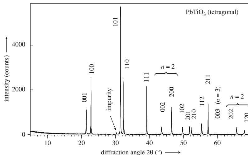
Fig. 4.47 Example of an experimental X-ray diffraction pattern. Recorded for a polycrystalline powder specimen of \text{PbTiO}_3 (tetragonal) using \text{Cu K}\alpha_1 radiation. At specific values of the diffraction angle 2\theta diffracted intensity can be observed. Consequently, the diffraction pattern can be conceived as a “fingerprint” of the diffracting substance. Such phase identification concerns one of the main applications of X-ray diffraction in materials science (measurement by Dr. A. Leineweber, Max Planck Institute for Metals Research)
