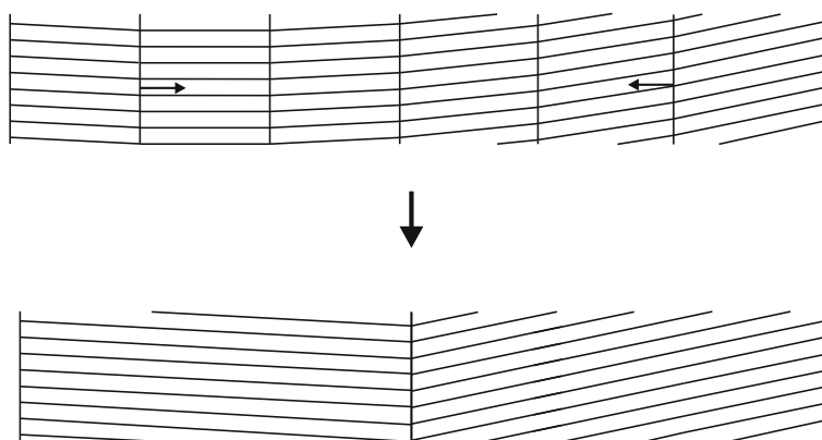
Fig. 10.9 Subgrain coarsening in an orientation gradient. In the case considered, upon traversing a grain in the polygonized microstructure, there may be a systematic trend in the orientation variation of the subgrains: while maintaining the minor magnitude of the variation of the orientation at each subgrain boundary, the systematic (minor) change of orientation can occur in the same direction, and as a result the difference in orientation of the “first” subgrain and the “last” subgrain met along the passage can be relatively large. If subgrain coarsening starts at distant locations along the passage considered, the formation of a higher angle grain boundaries is possible as sketched in the figure
