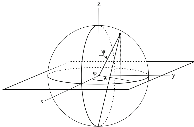
Fig. 4.52 Definition of the angle \psi , the specimen tilt angle, and the angle \varphi , the angle of rotation around the normal of the surface of the specimen. A (\psi, \varphi) combination denotes a direction in the specimen ( \psi = 0 denotes the surface-normal direction). Every (\psi, \varphi) combination indicates a certain direction in the specimen which intersects the sphere. The points of intersection on the upper hemisphere can be projected according to the stereographic projection (Fig. 4.48) onto the plane of projection which is the horizontal plane of the sphere (surface of the specimen). The intensity of a HKL reflection recorded for the (\psi, \varphi) direction can be indicated at every (\psi, \varphi) point in the SGP. The result is called a pole figure ; see Figs. 4.53, 4.54 and 4.55
