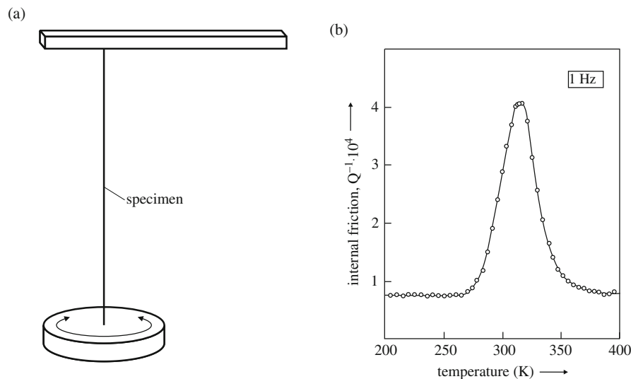
Fig. 11.14 (a) Schematic representation of a torsional pendulum. (b) The energy loss per cycle, proportional to a dimensionless quantity Q^{-1} usually applied as measure for internal friction and plotted along the ordinate, for a cycle frequency of 1 Hz (i.e. one cycle per second), as a function of temperature for b.c.c. iron containing interstitially dissolved carbon (here a ferritic steel): the Snoek effect. The peak height is a measure for the amount of carbon dissolved in the b.c.c. phase and from the result shown here it follows that about 20 at.ppm C is dissolved in ferrite; the detection limit of this method is about 1 at.ppm! From the temperature dependence of the frequency of maximal damping (i.e. the position of the maximum of the Snoek peak as shown in the figure is determined for various frequencies), diffusion data (the activation energy) of interstitially dissolved components can be determined with very high precision; cf. Sect. 8.5 (redrawn from Weller M (2006) Mater Sci Eng A 442:21–30)
