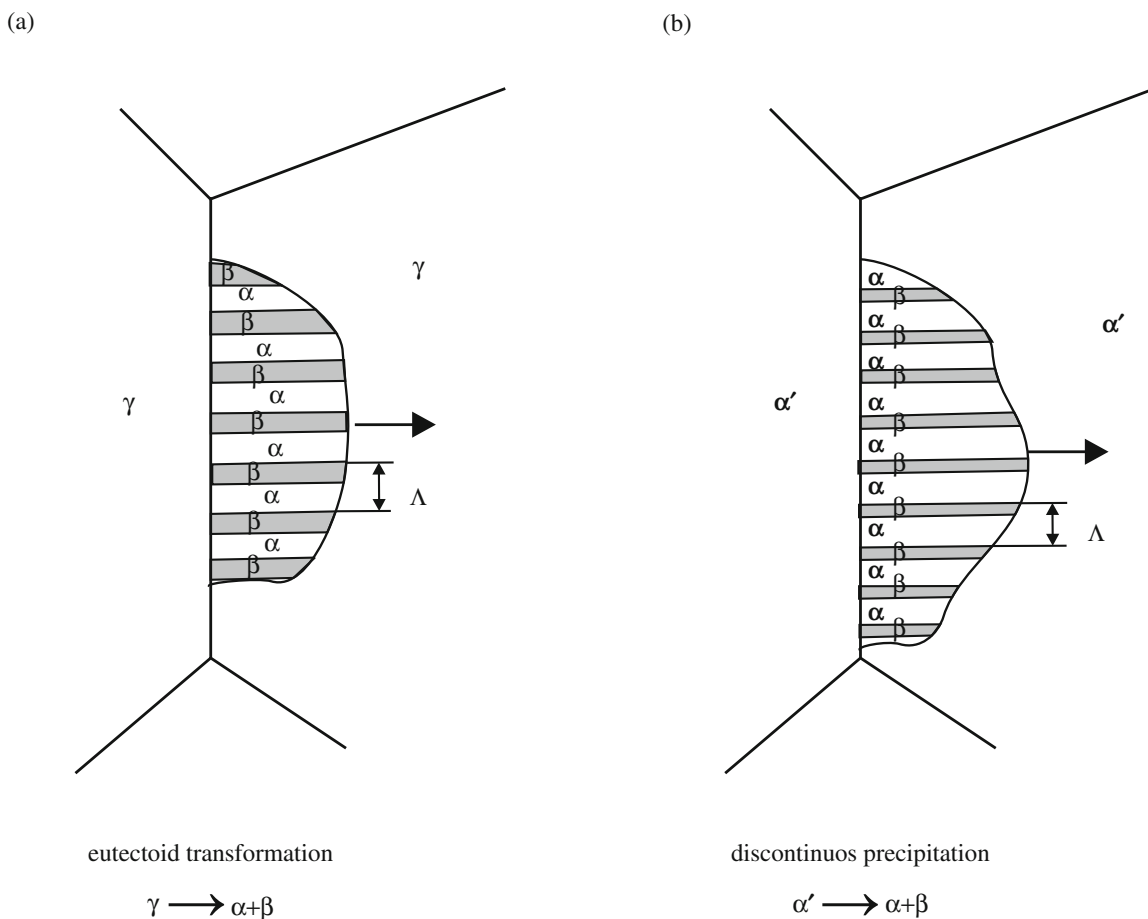
Fig. 9.8 Lamellar transformation product microstructures developing by growth from a grain boundary of the parent phase. (a) Schematic depiction of the reaction front of a eutectoid precipitation cell moving from a grain boundary into a grain of the parent phase \gamma . (b) Schematic depiction of the reaction front of a discontinuous precipitation cell moving from a grain boundary into a grain of the supersaturated matrix \alpha' . \Lambda is the period of the lamellar product structure
