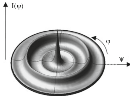
Fig. 4.55 The \{110\} pole figure of the surface of a b.c.c. Nb film of thickness 500 nm prepared by magnetron sputter deposition on a 500 \mu\text{m} thick single crystalline Si wafer, with a (510) surface, covered with a 50 nm thick amorphous \text{SiO}_2 layer. The preferred orientation is described as a \{110\} fibre texture, with the fibre axis parallel to the normal of the film surface. The intensity maximum at the centre of the \{110\} pole figure corresponds to crystals with \{110\} planes parallel to the surface. These same crystals also give rise to intensity maxima in the pole figure at those tilt angles \psi where the other members of the set of equivalent families of \{110\} planes diffract; further see Fig. 4.56 (taken from Okolo B, Lamparter P, Welzel U, Mittemeijer EJ (2004) J Appl Phys 95:466–476)
