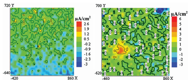
Fig. 4 Coating modified with a mixture of mercaptopbenzothiazole-loaded LDH and cerium molybdate nanocontainers. Current density maps obtained at immersion times in 0.05 M NaCl: after 3 h (left) and after 40 h (right). 43
